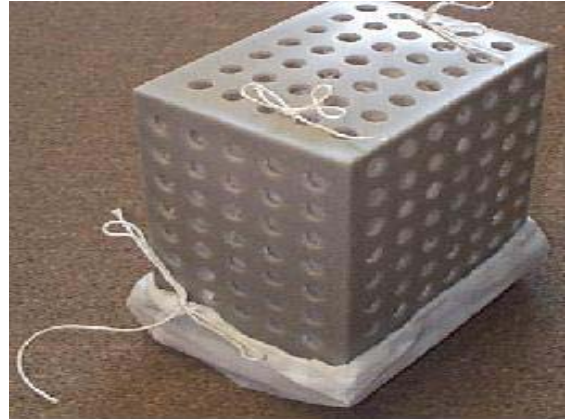
Tie filter bags to bottom of baskets
