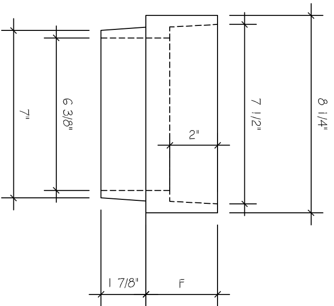
PAVING RING DETAIL
